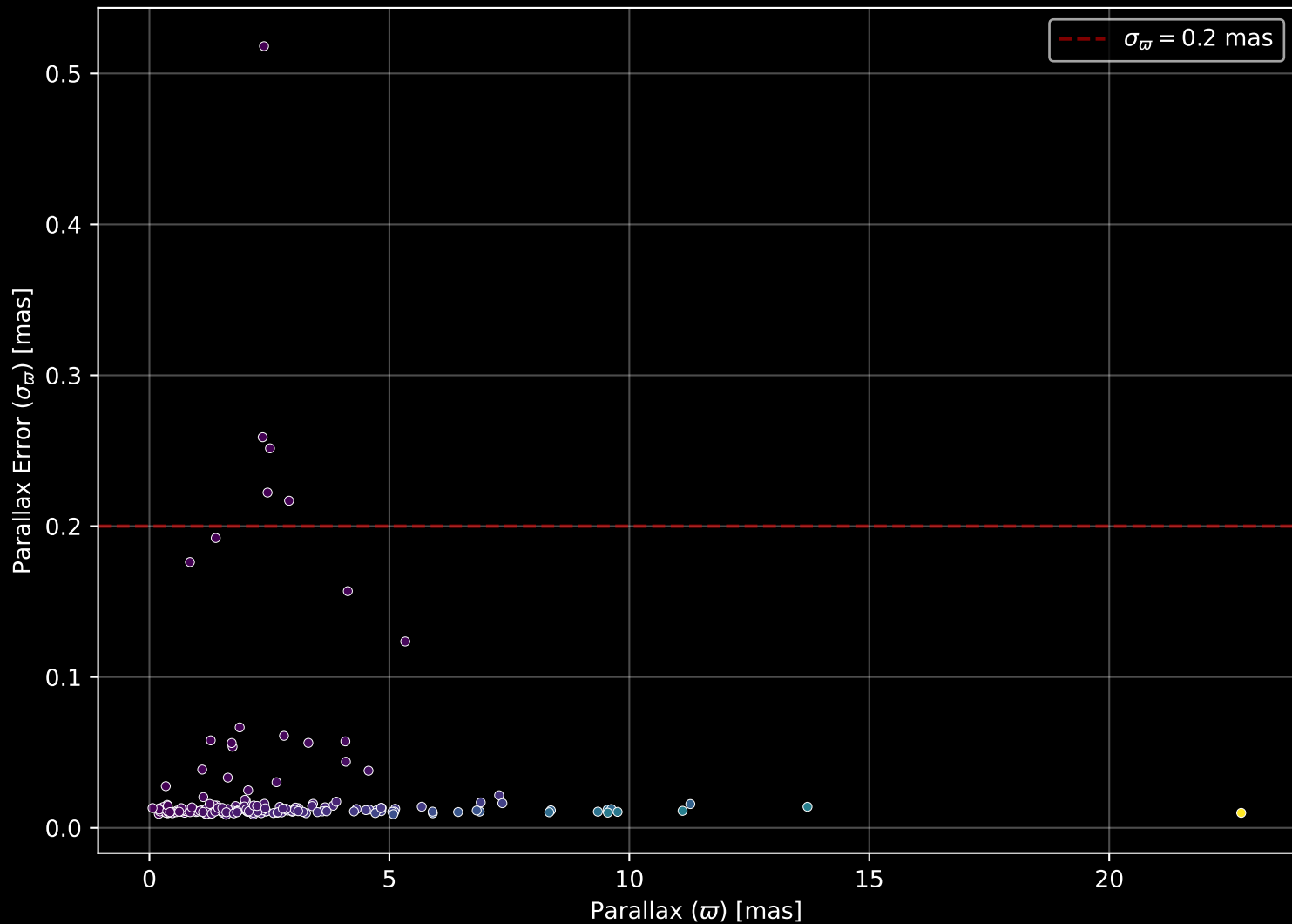
APOGEE DR17 Field: [274-39-O_TESS] Parallax Quality (n= 197)
