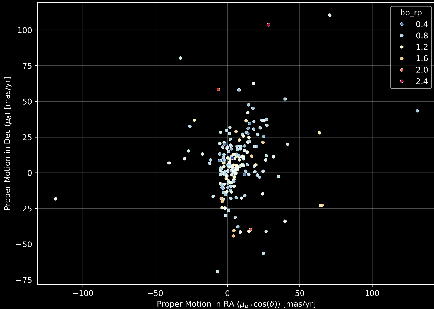
APOGEE DR17 Field: [274-39-O_TESS] Proper Motion Diagram (n= 197)
