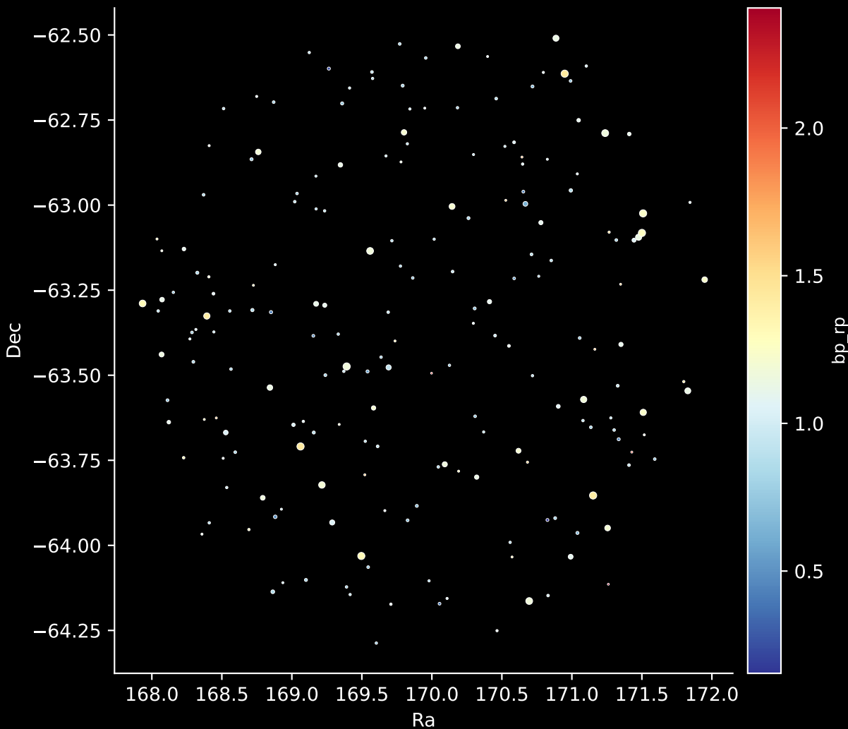
APOGEE DR17 Field: [274-39-O_TESS] Stars: 197
