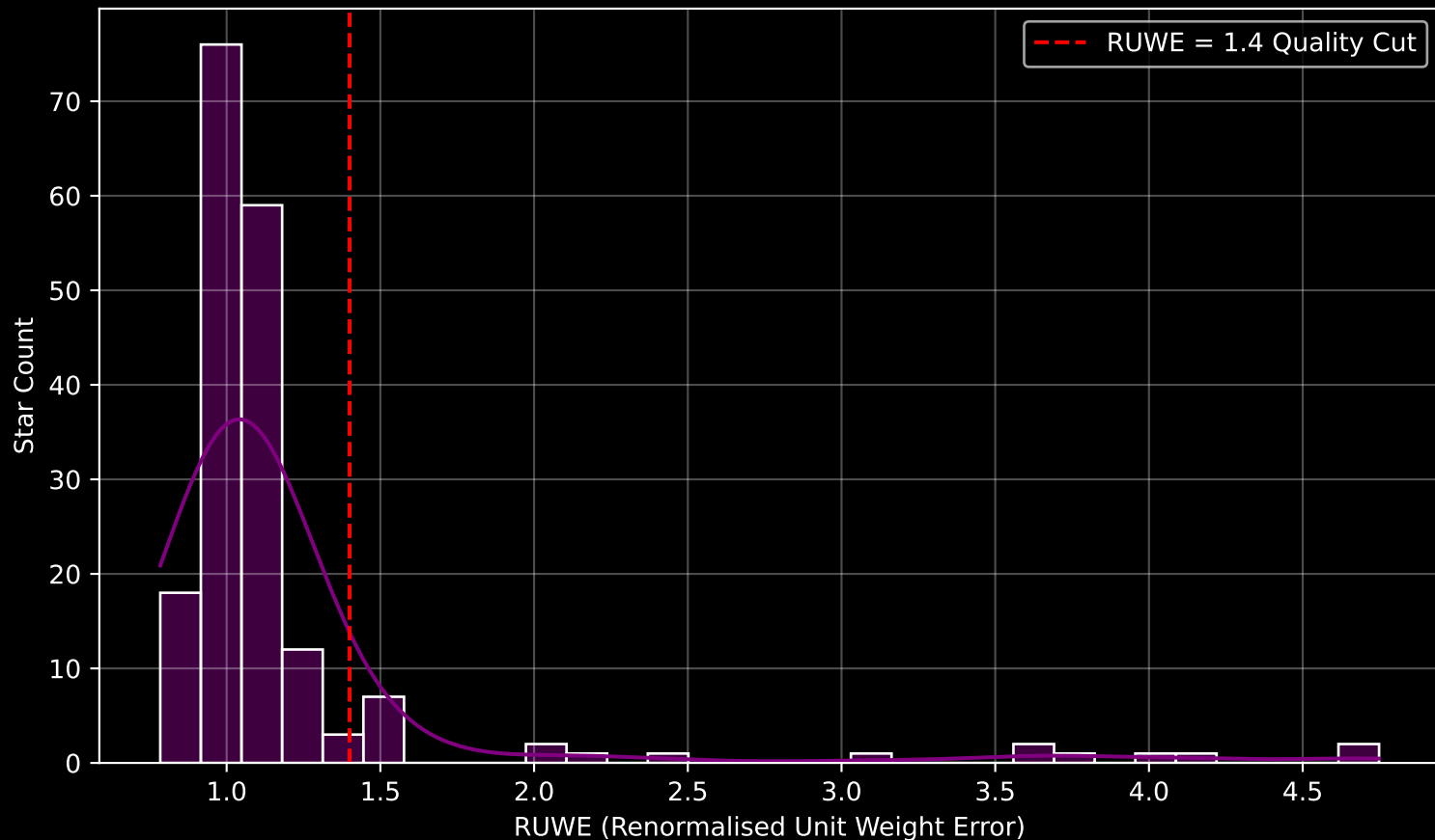
GAPOGEE DR17 Field [274-39-O_TESS] RUWE Distribution (n= 187)
