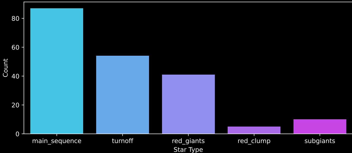
APOGEE DR17 Field: [274-39-O_TESS] Count plot of Star Type
