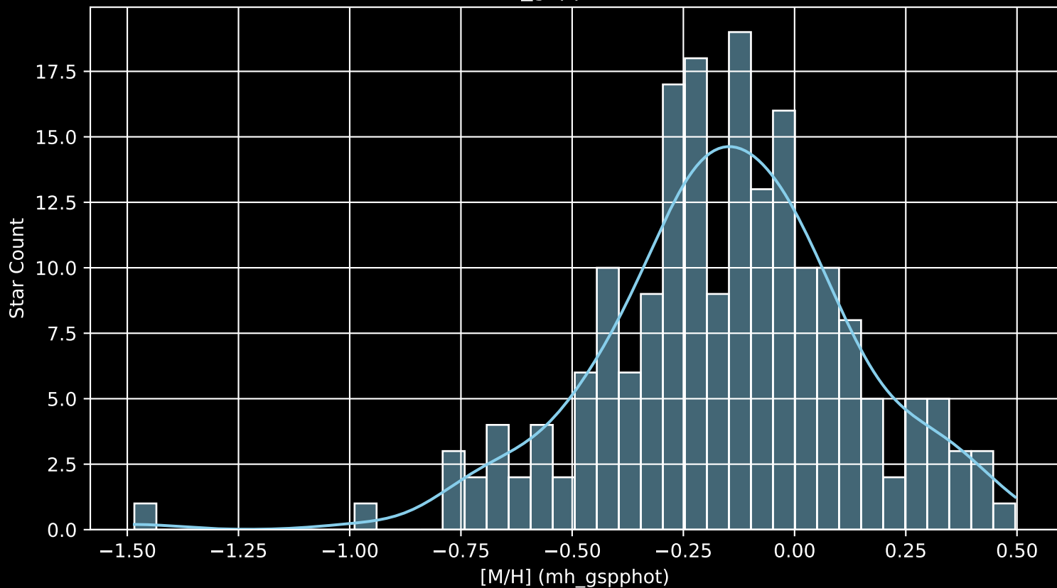
APOGEE DR17 Field: [274-39-O_TESS [M/H] (mh_gspphot) (n= 194)
