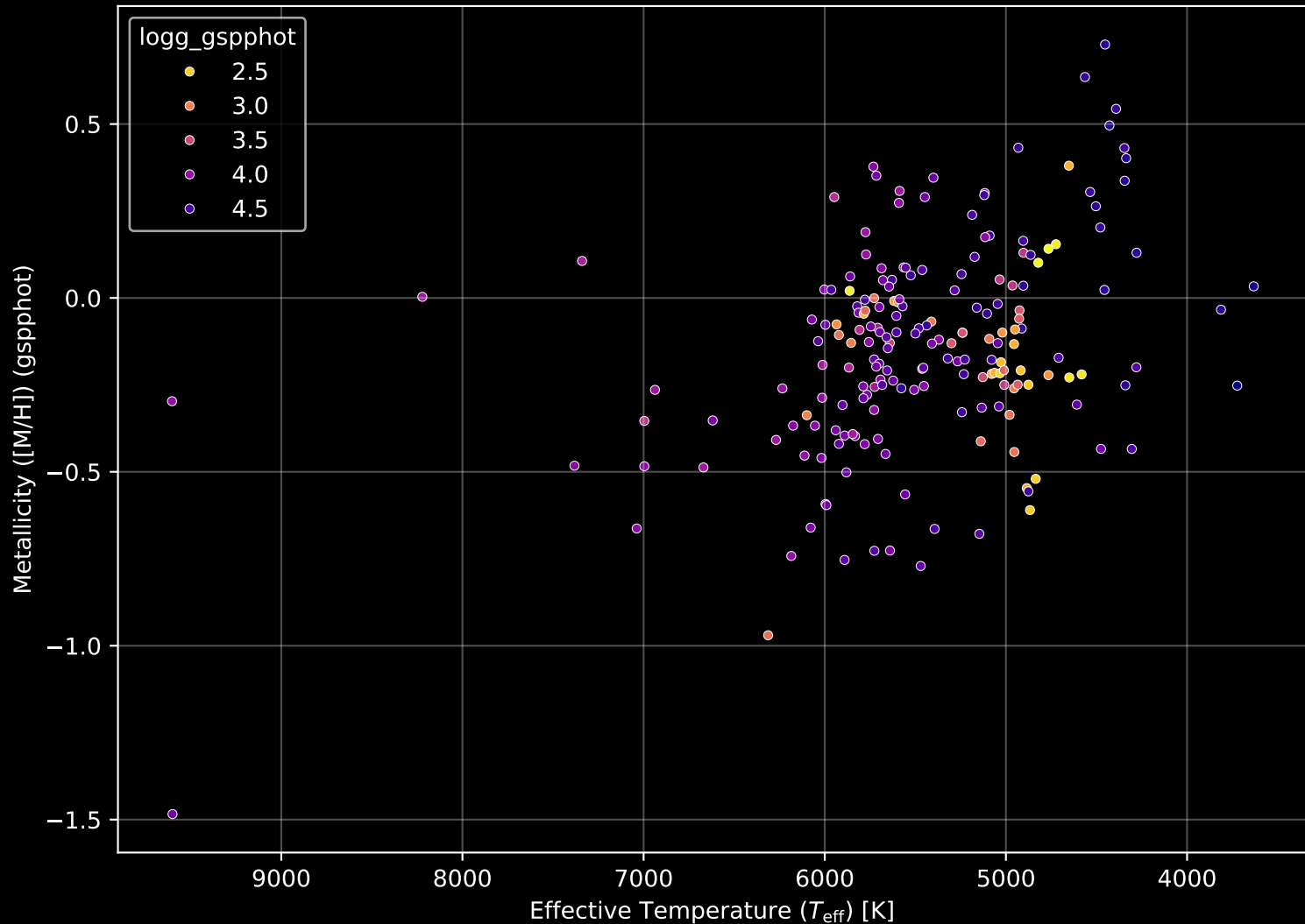
APOGEE DR17 Field: [274-39-O_TESS] Stellar Population Parameters (n= 197)
